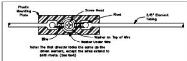
Figure 2—Drawing of the driven-element modification.
